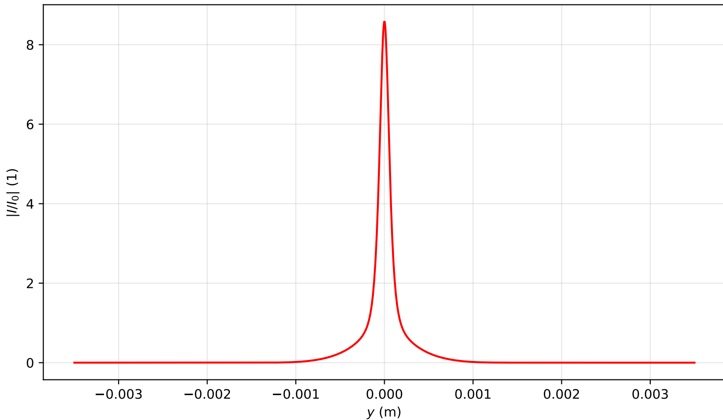
Intensity profile I(x=0, y, z=0.478)/I_0 , P_{in}=4.5P_{cr} , artificial time
